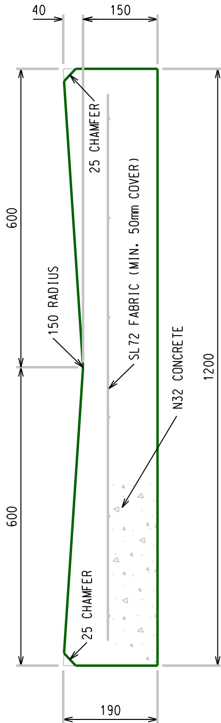
1200mm SPOON DRAIN
