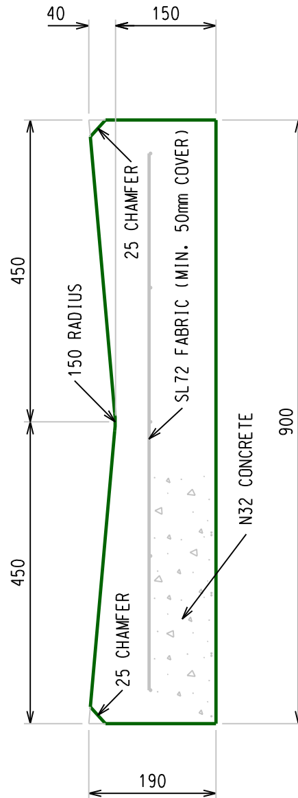
900mm SPOON DRAIN
