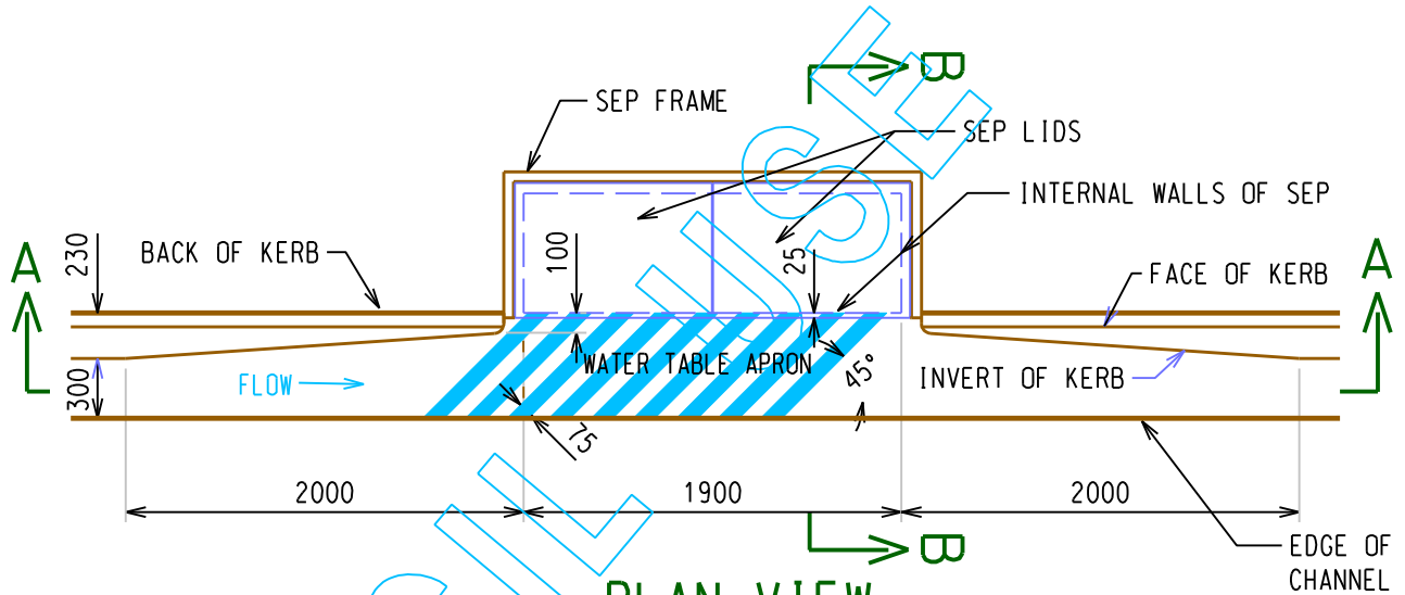
PLAN VIEW
